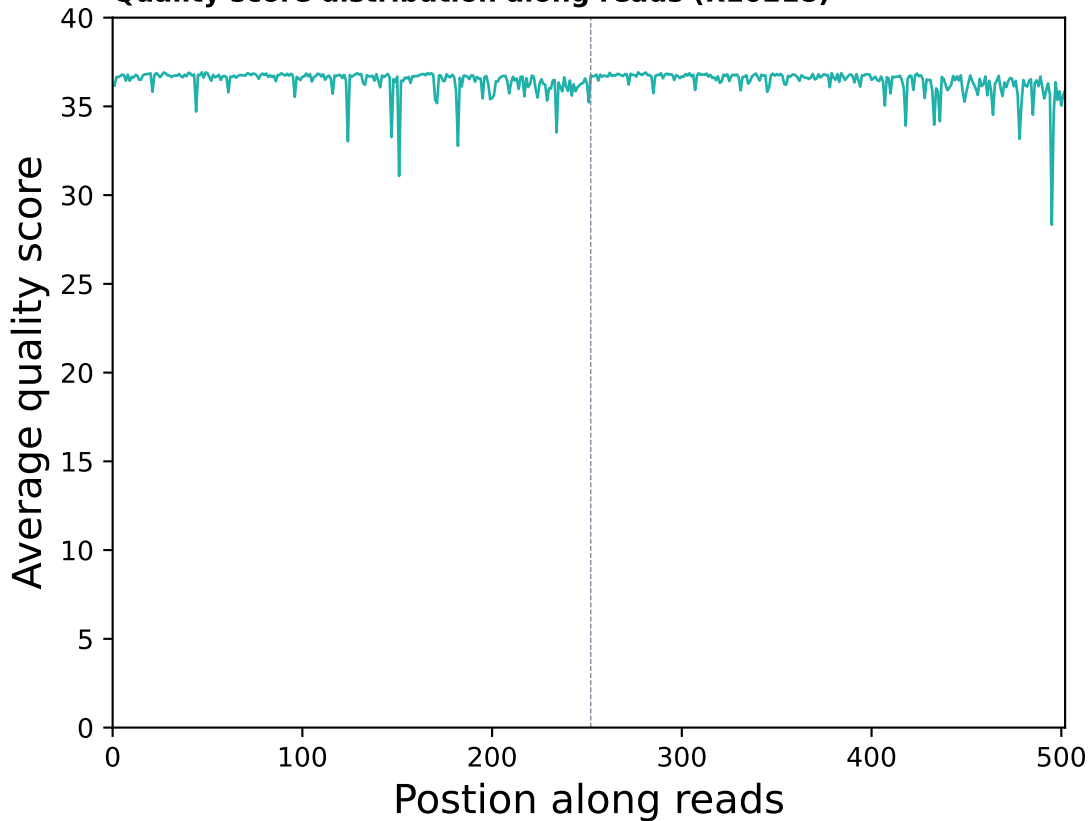
Quality score distribution along reads (R10218)
